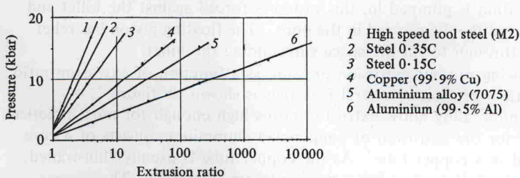
Figure 2. Pressure versus extrusion ratio for some common materials.
